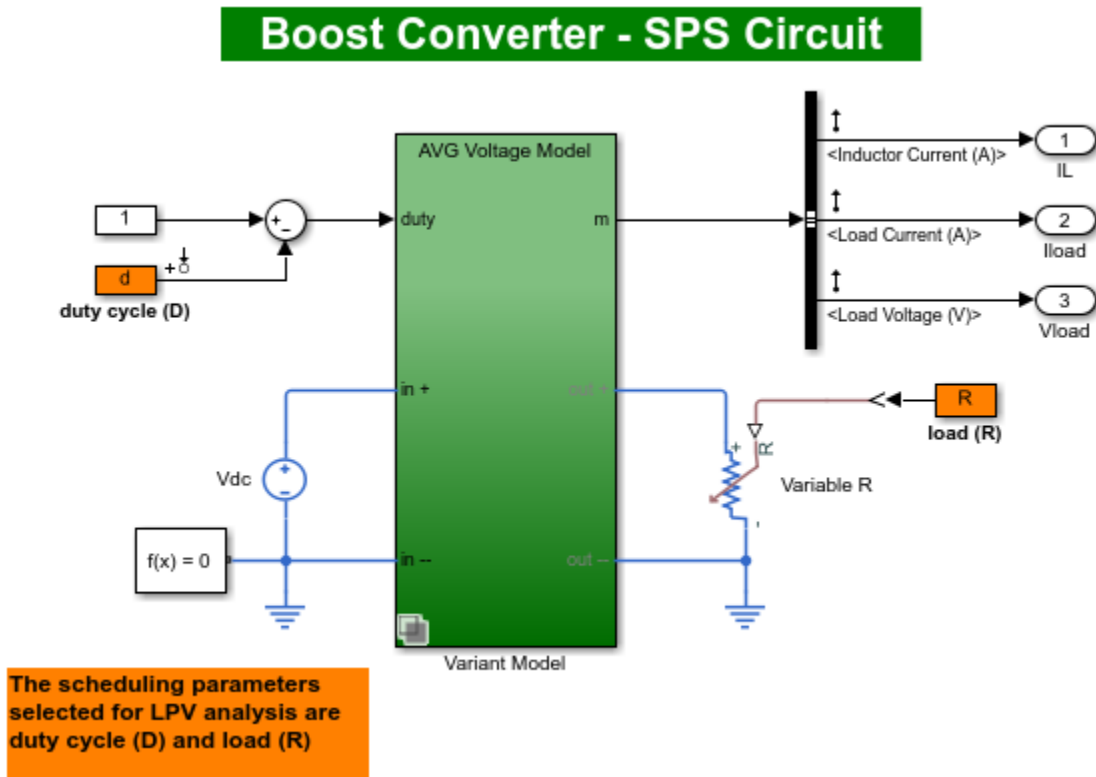
Figure 2: Simscape Electrical based Boost Converter model
