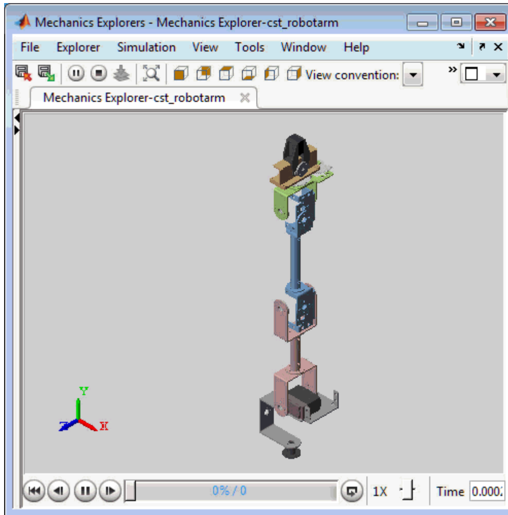
Figure 9: Fine-tuned response.
